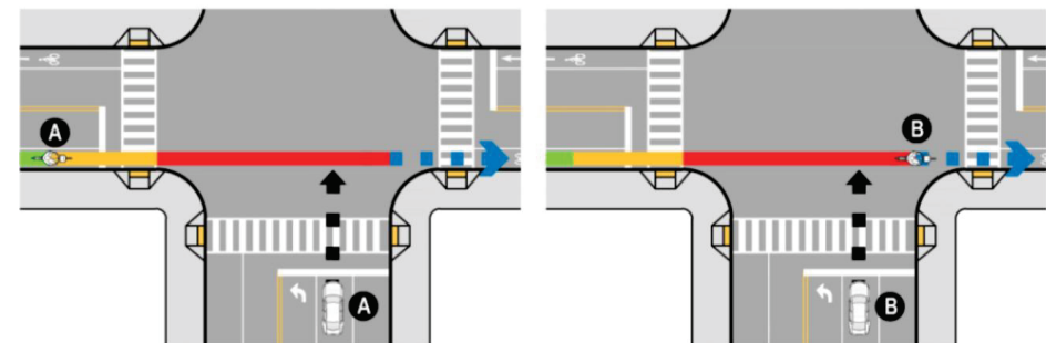
Bicycle Position with 5-second Red Clearance
